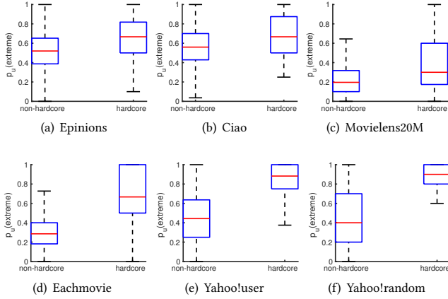
Figure 2: Ratio of 1, 5 ratings ( p_u(extreme) ) for hardcore and non-hardcore users in various datasets.
